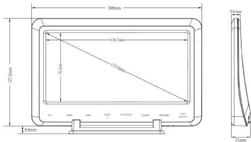
Figure 2: Size
