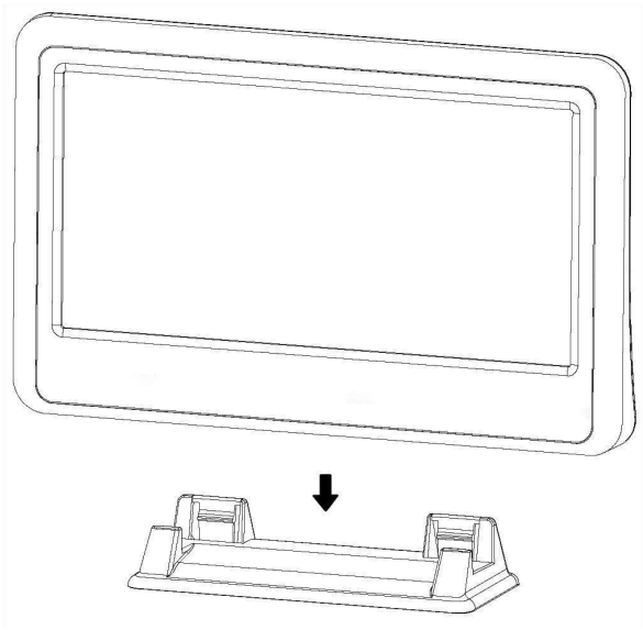
Figure 1: Install Bracket
